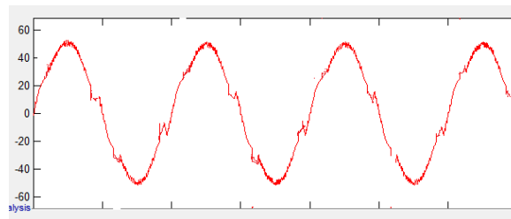
Figure 7. Resultant line current after current compensation
