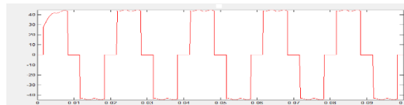
Figure. 4. Distorted line current
