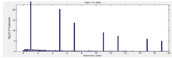
Figure 5. THD analysis of distorted current waveform
