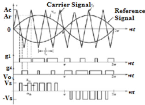
Fig. (b) Sinusoidal pulse width modulation
