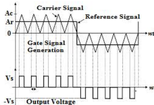
Fig. (a) Multiple pulse width modulation
