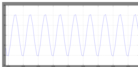
Fig.(k) Waveform of output current flowing in resonance circuit.
