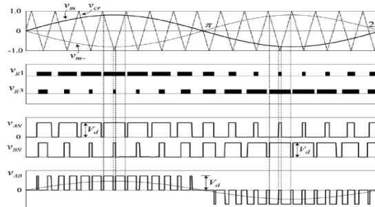
Fig.(d) waveform of PWM with Unipolar Voltage Switching
