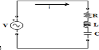
Fig.(i)Series resonance circuit
