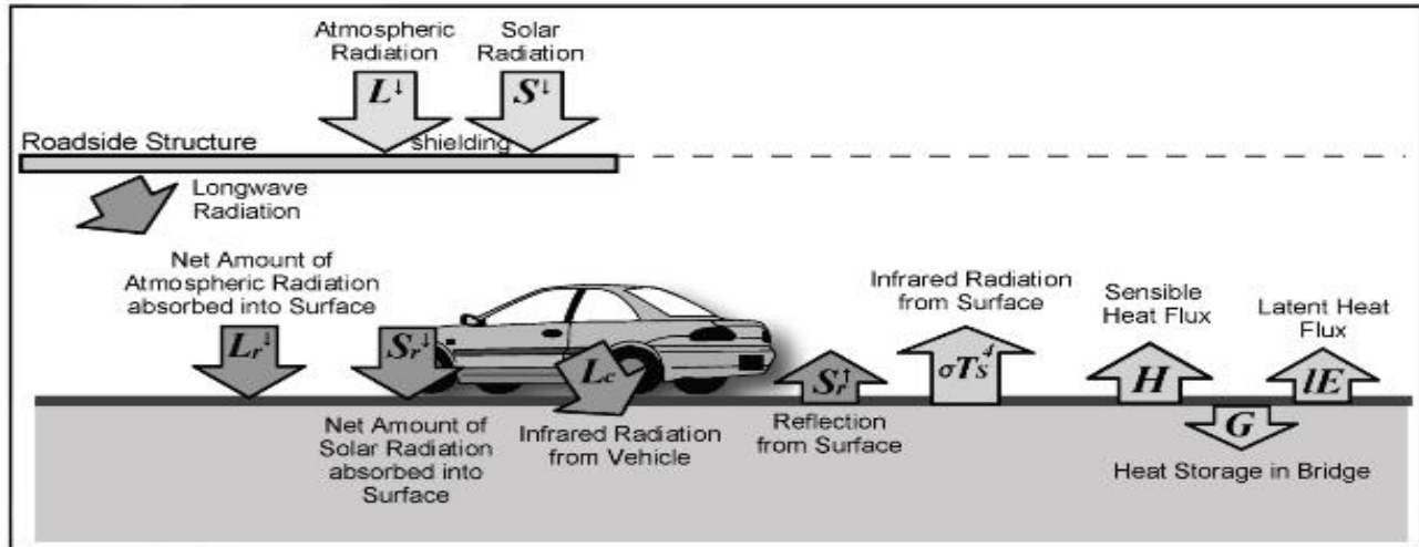
Figure 3 3.Road Surface Temperature Prediction Model(Takahashi, 2008)
