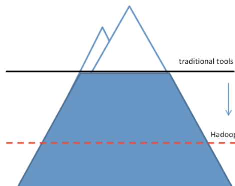
Fig 1: Hadoop Level
