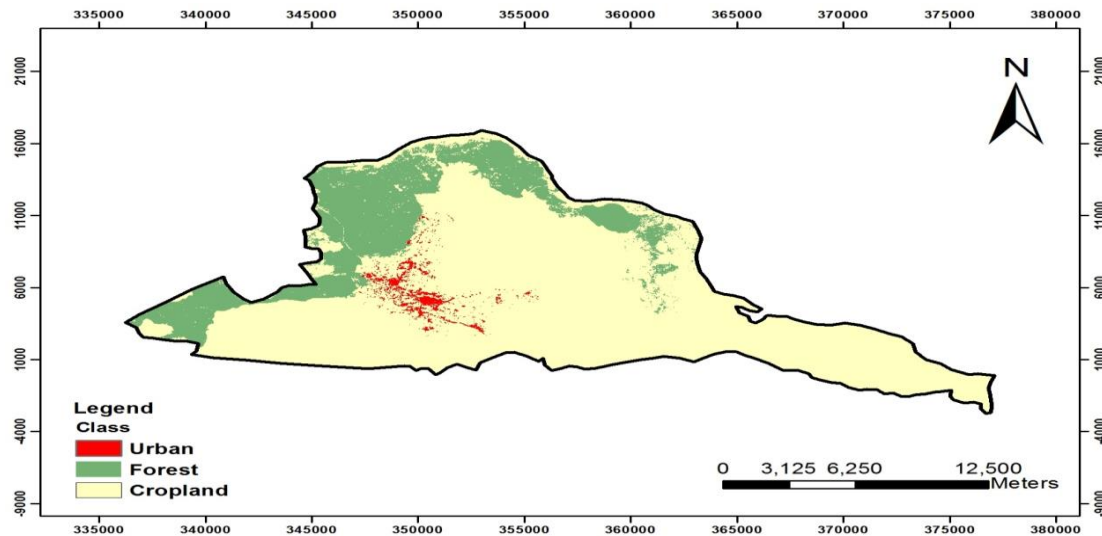
Figure 4.2 Classified image, 2000.
