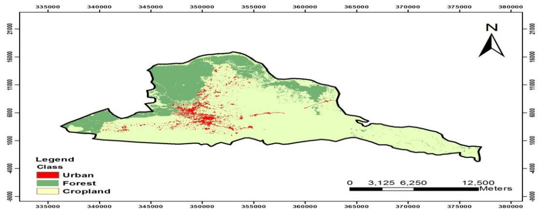
Figure 4.3 Classified image, 2014.
