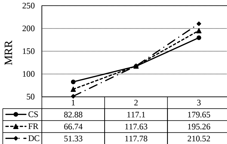
Figure 7: Effect of various turning parameters on MRR
