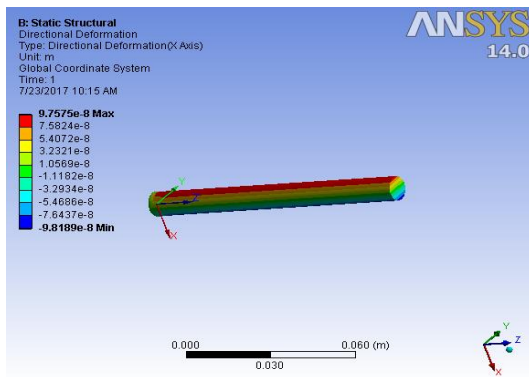
Figure-10 Directional deformation (MS300)
