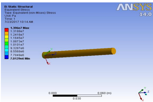
Figure-6 Equivalent (Von-mises) stress (MS300) (Composite)
