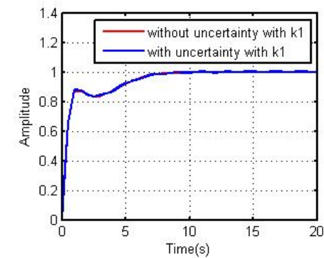
Figure 5: Step response of the plant using k_1 with and without uncertainty
