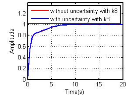
Figure 9: Step response of the plant using k_8 with and without uncertainty
