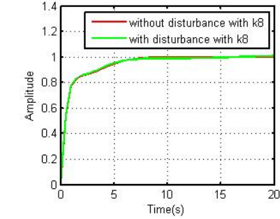
Figure 10: Step response of the controlled plant using k_8 with and without disturbance
