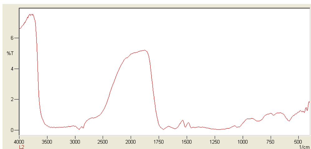
Fig. 6 FTIR spectrogram for L-2
