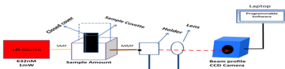
Figure 1: The experimental configuration block diagram.
