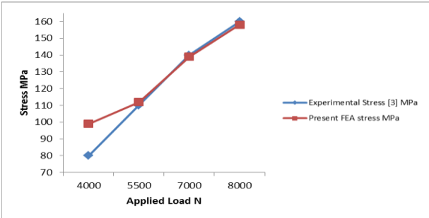
Fig. 8 Comparison of Present FEA result and Experimental Study
