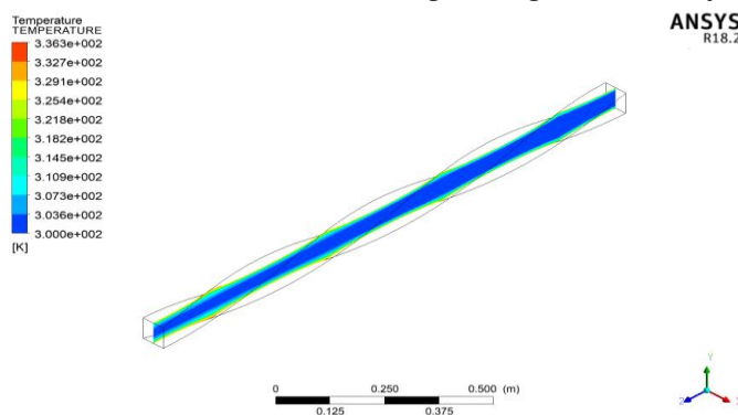
Fig. 4.6 Effect of twisted square duct at a velocity of 4.5 m/sec
