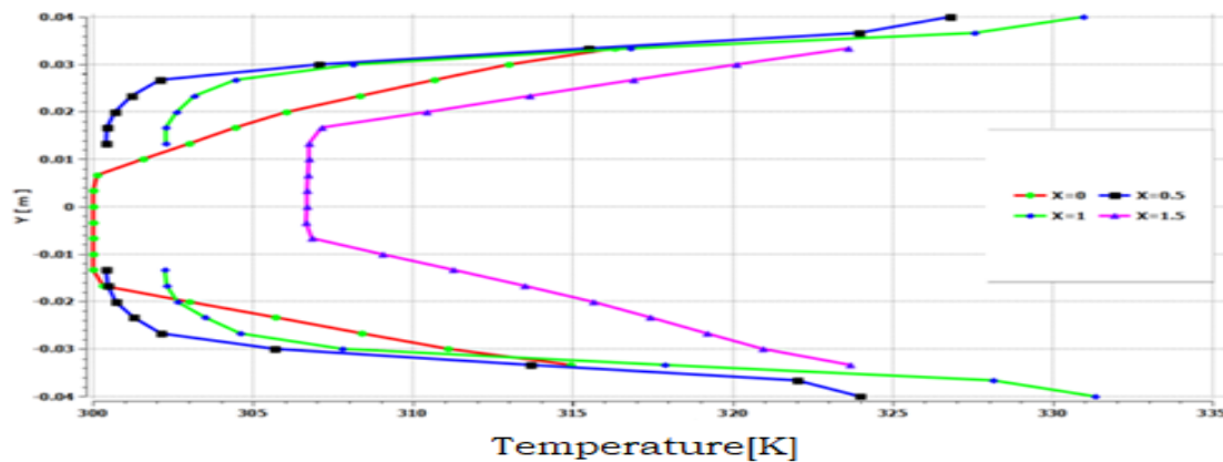
Fig . 4.12 Temperature profile of twisted circular rod at a velocity of 4.5 m/sec.
