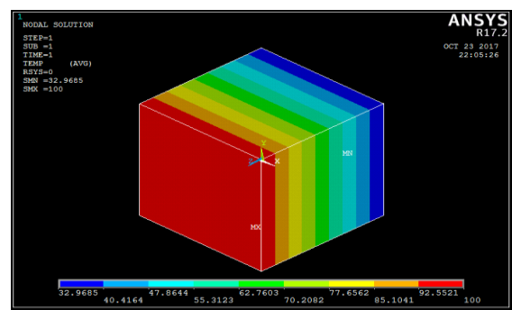
Fig-8: 10 Wt % of Titanium oxide Filler
