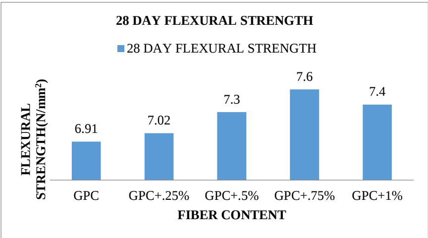
Fig 3.3Flexural strength results
