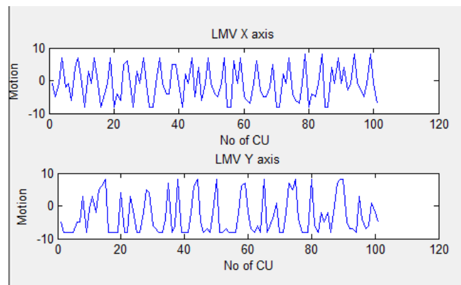
Fig.5. Extract Feature
