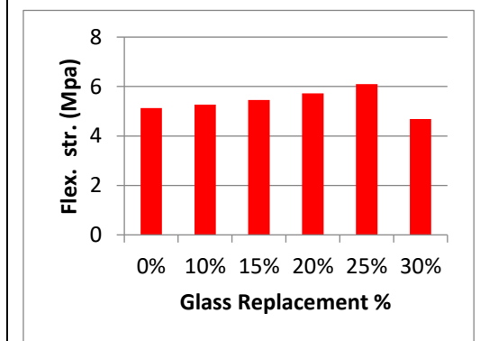
Fig. 6: Flex Str of FWGAC 28 days
