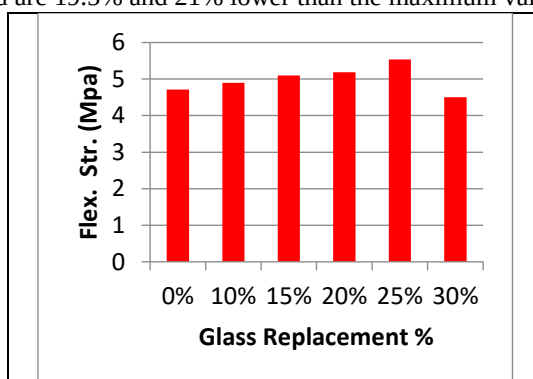
Fig. 5: Flex Str of FWGAC 7 days
