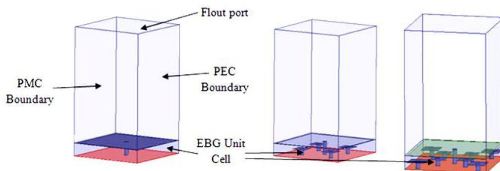
Figure 2: Simulation setup for measurement of coefficient of reflection for three EBG models
