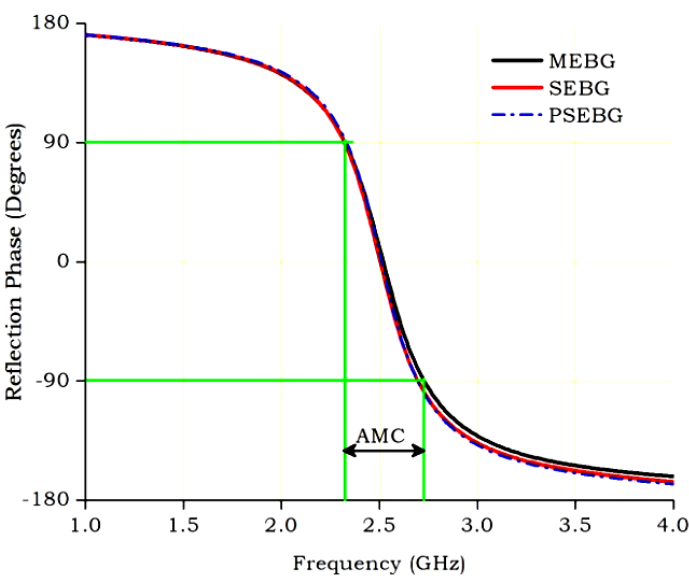
Figure 3: Reflection phase diagram
