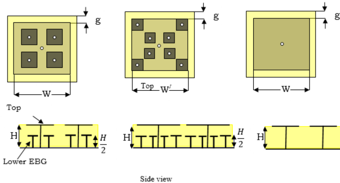
(a) Stacked EBG, (b) Progressive stacked EBG (c) Mushroom type EBG (reference model), Figure 1: schematics of EBG structures
