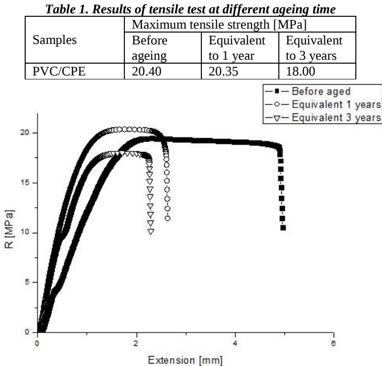
Figure 1. Result of tensile test
